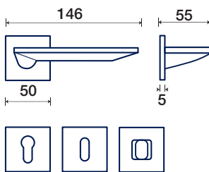
rosette - bocchette 5 mm rosettes - escutcheon
